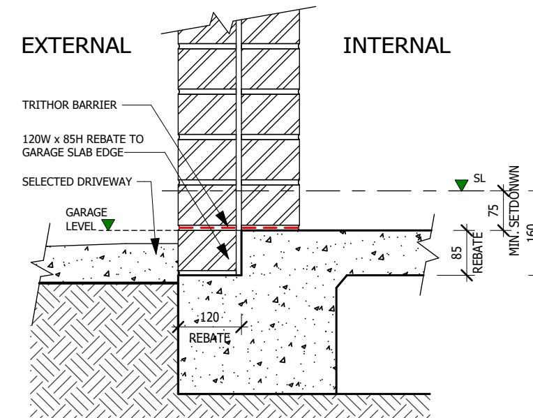
2 GARAGE REBATE (FRONT SIDE OF DOOR)
