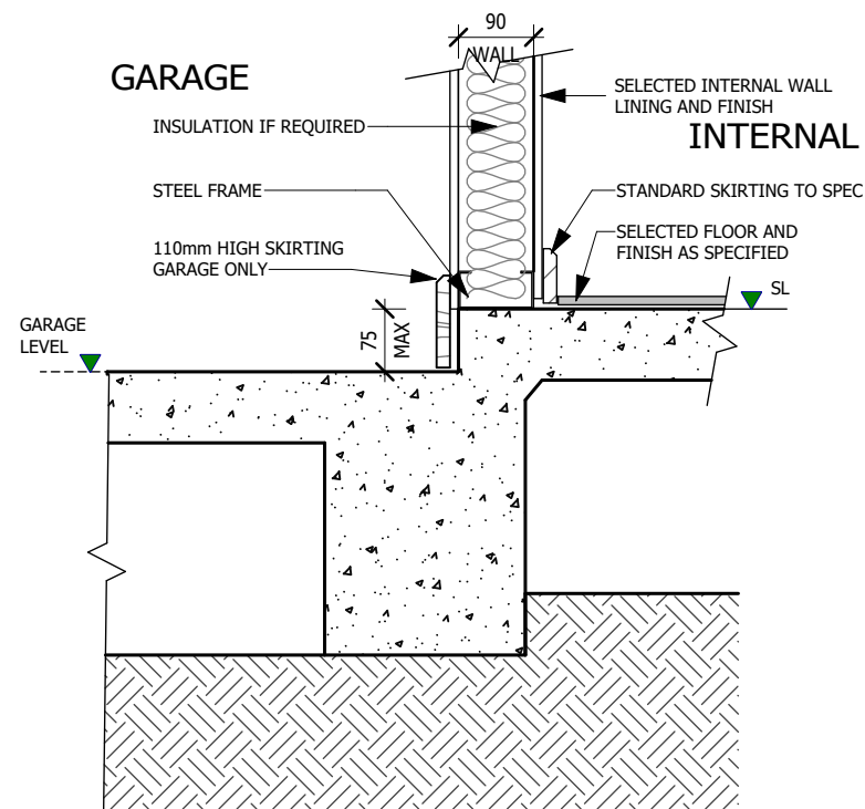
4 INTERNA GARAGE STEP - 75MM STEP ONLY SCALE: 1 : 10
