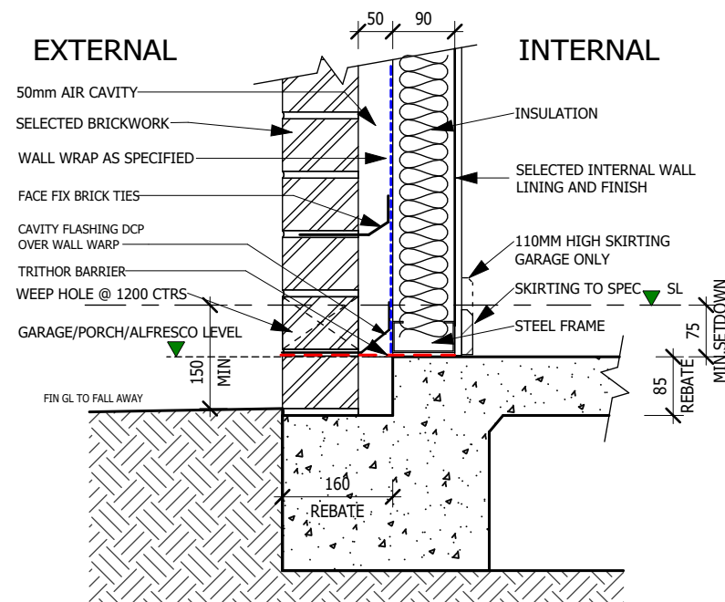
1 GARAGE REBATE (SIDE) & PORCH/ALFRESCO
