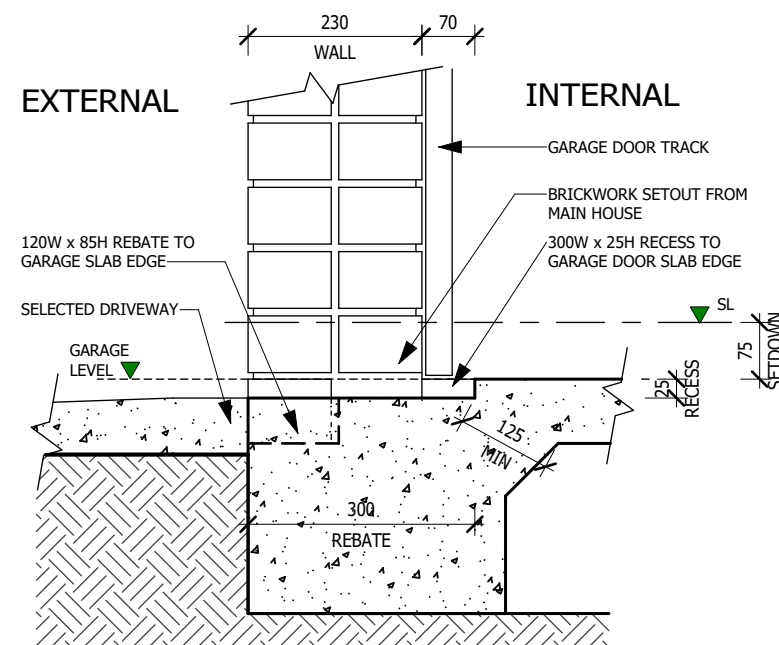
3 GARAGE RECESS (FRONT THROUGH RECESS)
