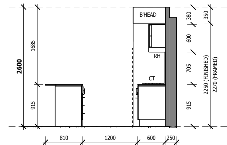
ELEVATION K4
