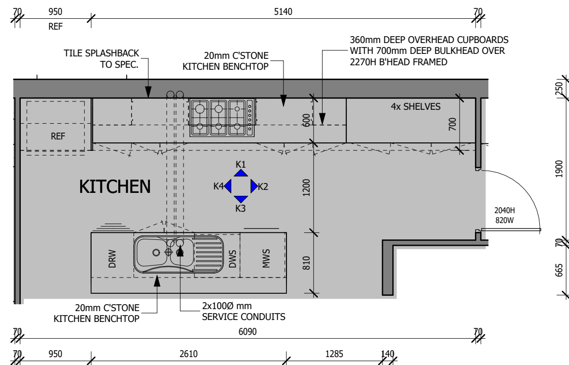
KITCHEN PLAN
